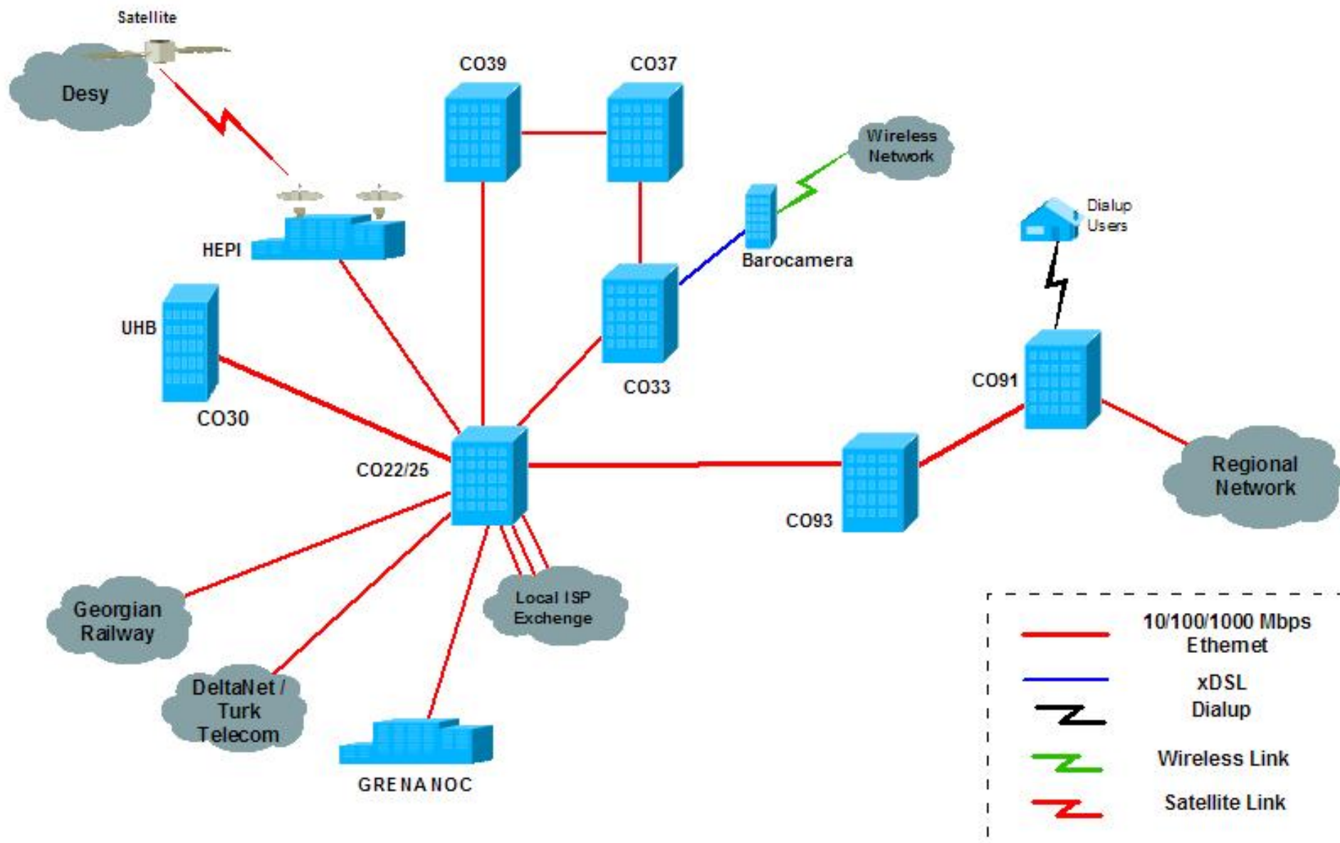
Scheme of the Georgian segment of GUAM information space
